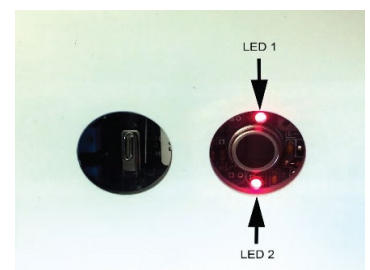
Figure 2-2 LEDs
