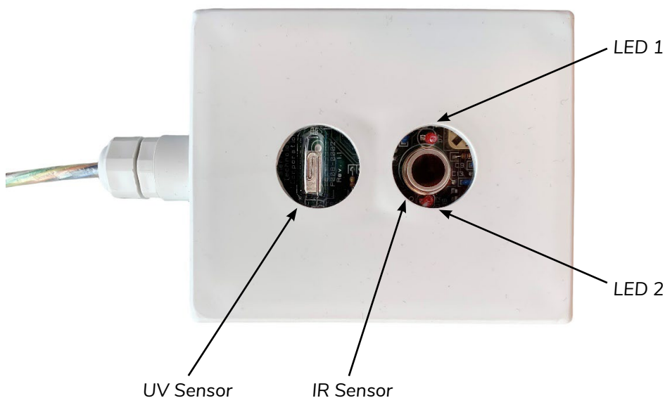
Figure 7-2 DCR1 Layout (Sensors & LEDs)
