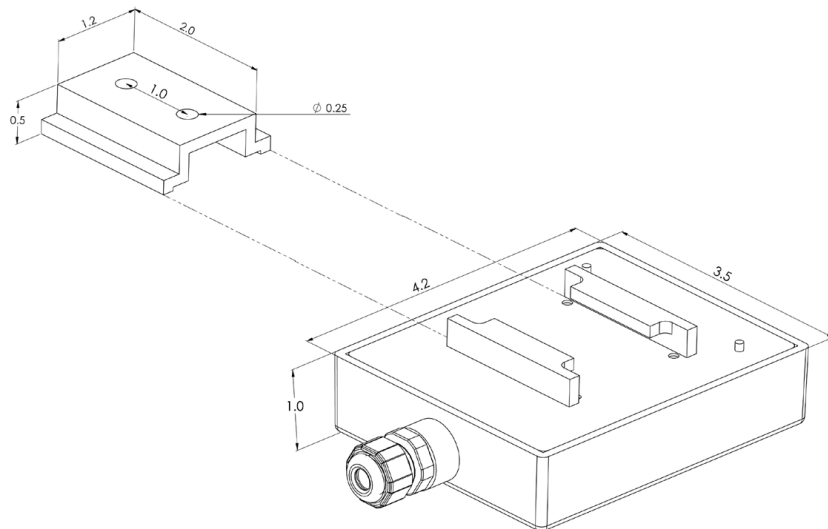
Figure 7-1 DCR1 Housing Dimensions
