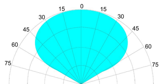
Figure 2-1 Field-of-View
